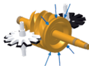
Radial loads act on both the top and underside of the main rotor.
